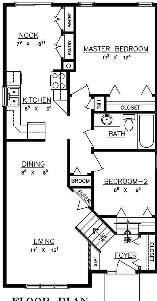
FLOOR PLAN
